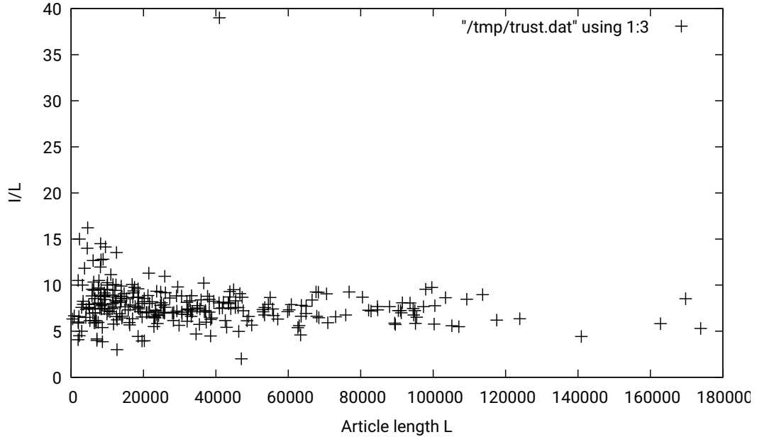
Figure 3: The scaled contention per unit length is noisily constant. This is interesting because it implies that contention is not related to subject but to groups a shared process, i.e. human interaction. There is more noise in the measures for smaller articles due to the coarseness of rescaling.
