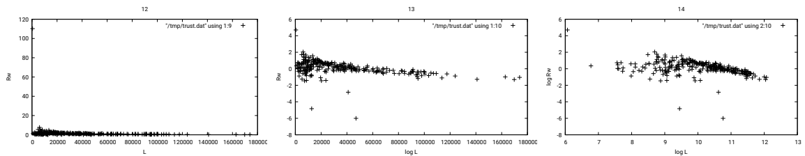
Figure 8: Edit rate per unit length of article H/L relaxation of edit changes per article length as raw, log, and log-log plots. This potentially tells us that the growth or decay of the edit process with time. However, it's unclear whether this is an exponential decay or a power law. Both graphs are equally noisy. There is more contention per unit length for small articles, as an artifact of scaling and novelty. There's no strong straight-line relationship in any of the versions of the graph.
