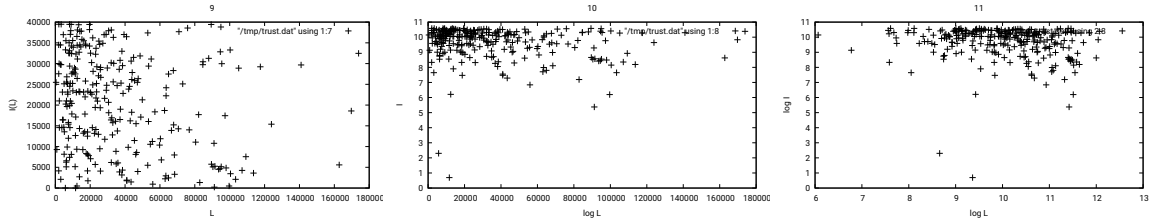
Figure 7: Contention as a function of article length (partial proxy for time) I(L) in three graphs: I versus L on the left, I versus \log(L) , and \log(I) versus \log(L) . The log-log plot seem most compact, suggesting a general power law relationship, which is also expected on probabilistic grounds. This tells us (again) that the tendency for contention is independent of time or subject: it's a basic human phenomenon.
