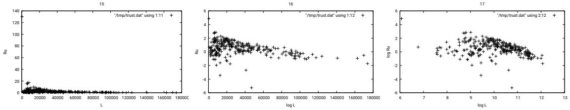
Figure 9: Trusted sample set s/S relaxation of edit changes per trusted article sample. This can be compared with figure 8. The similarity between the graph shows that trusting is justified in capturing the same average level of contention as in the full analysis. In other words, we don’t necessarily miss much by failing to micro-manage the process as a third party observer.
