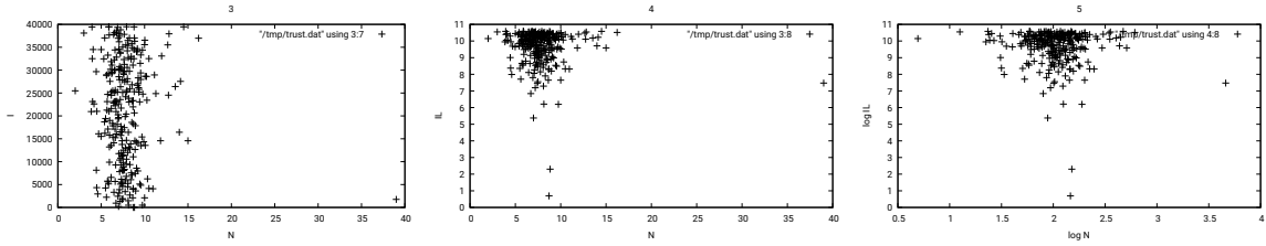
Figure 5: I(\langle N \rangle) , the dependence of contention in shared editing as a function of the average number of users per episode of editing. Editing is episodic or bursty and not all users are involved in every burst.
