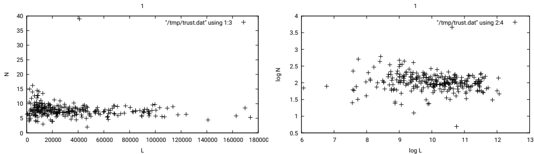
Figure 4: Relationship between user contributors per episode and article length, as pure \langle N \rangle(L) on the left and a log-log version on the right. The number of users per unit length is noisily constant.
